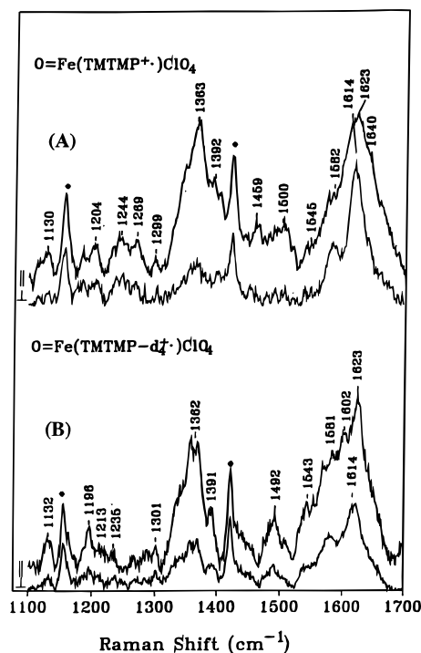
Figure 6. The high-frequency resonance Raman spectra of (A) O=Fe IV (TMTMP + )ClO 4 and (B) O=Fe IV (TMTMP- d 4 + )ClO 4 obtained with parallel and perpendicular polarization. Samples were measured in CH 2 Cl 2 at -80 °C with excitation at 406.7 nm. Bands marked with asterisks are due to solvent bands.
