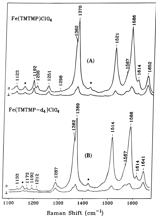
Figure 3. The high-frequency polarized resonance Raman spectra of \text{Fe}^{\text{III}}(\text{TMTMP})\text{ClO}_4 (trace A) and \text{Fe}^{\text{III}}(\text{TMTMP-}d_4)\text{ClO}_4 (trace B) measured in \text{CH}_2\text{Cl}_2 at room temperature with excitation at 406.7 nm.
